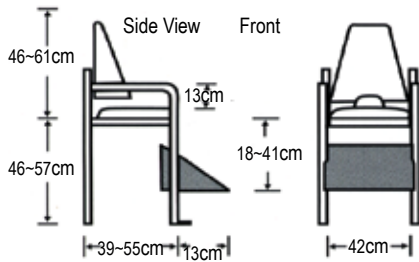
Dimensions of Positioning Commode
